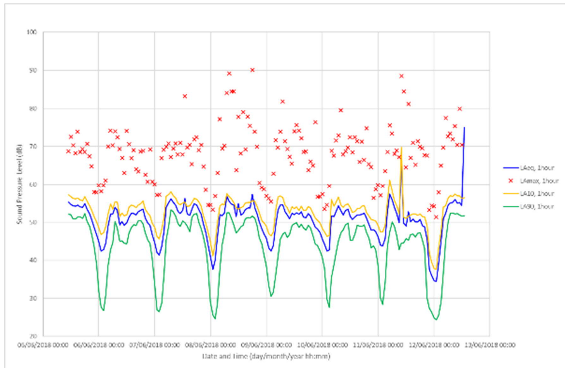
Figure 11.3.3 LT3 plot of results
